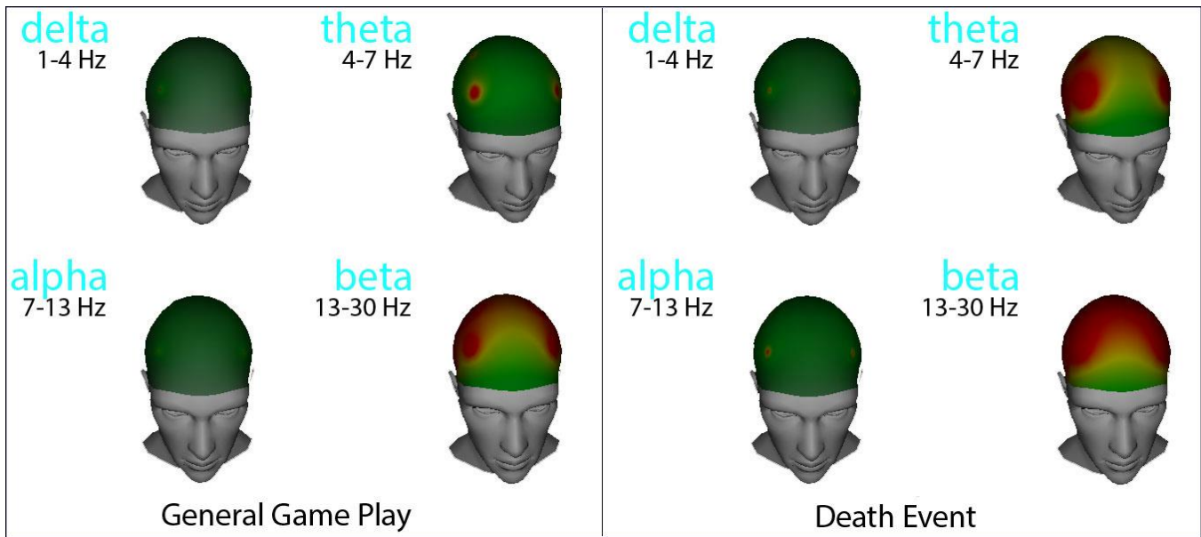
Figure 3. Brain activity during general game play and death events.
